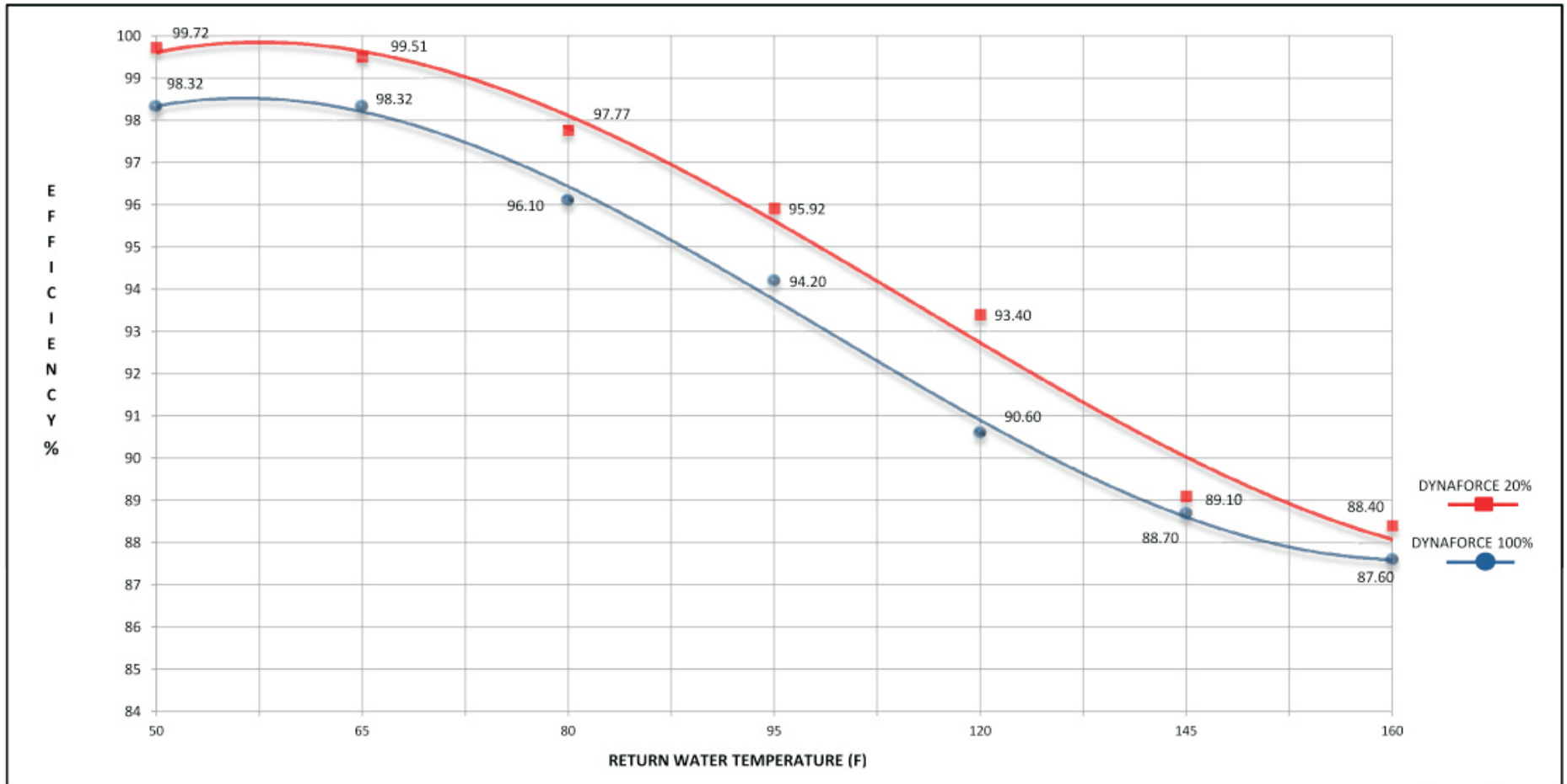
DYNAFORCE - 20% and 100% Fire Rate BOILER THERMAL EFFICIENCY
