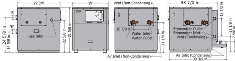
Side View (Left) Front View Side View (Right) Side View (Right) Condensing
